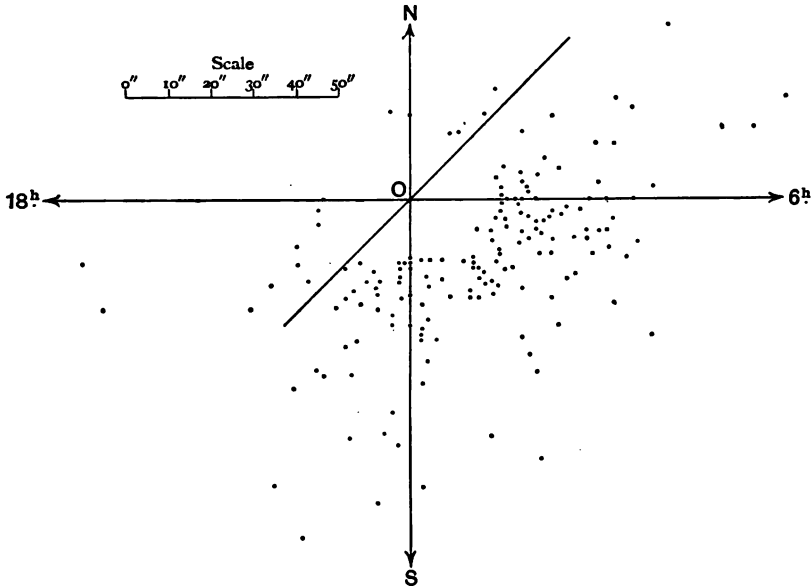
FIG. 13.—Distribution of Large Proper Motions (Dyson).
